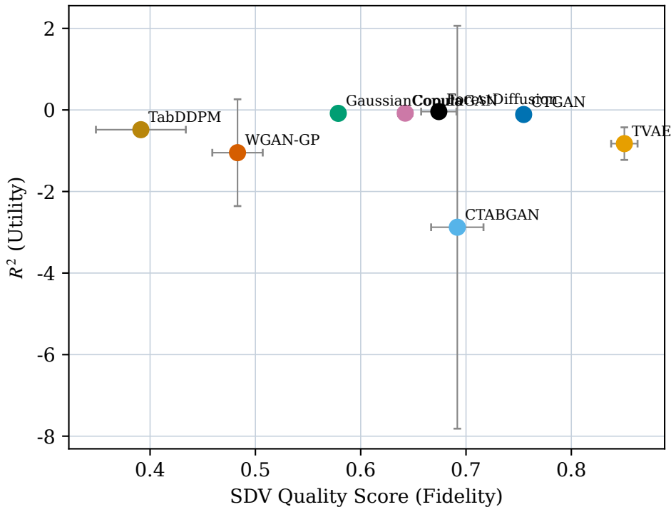
Metro Interstate: SDV Quality Score (Fidelity) vs R^2 (Utility)
